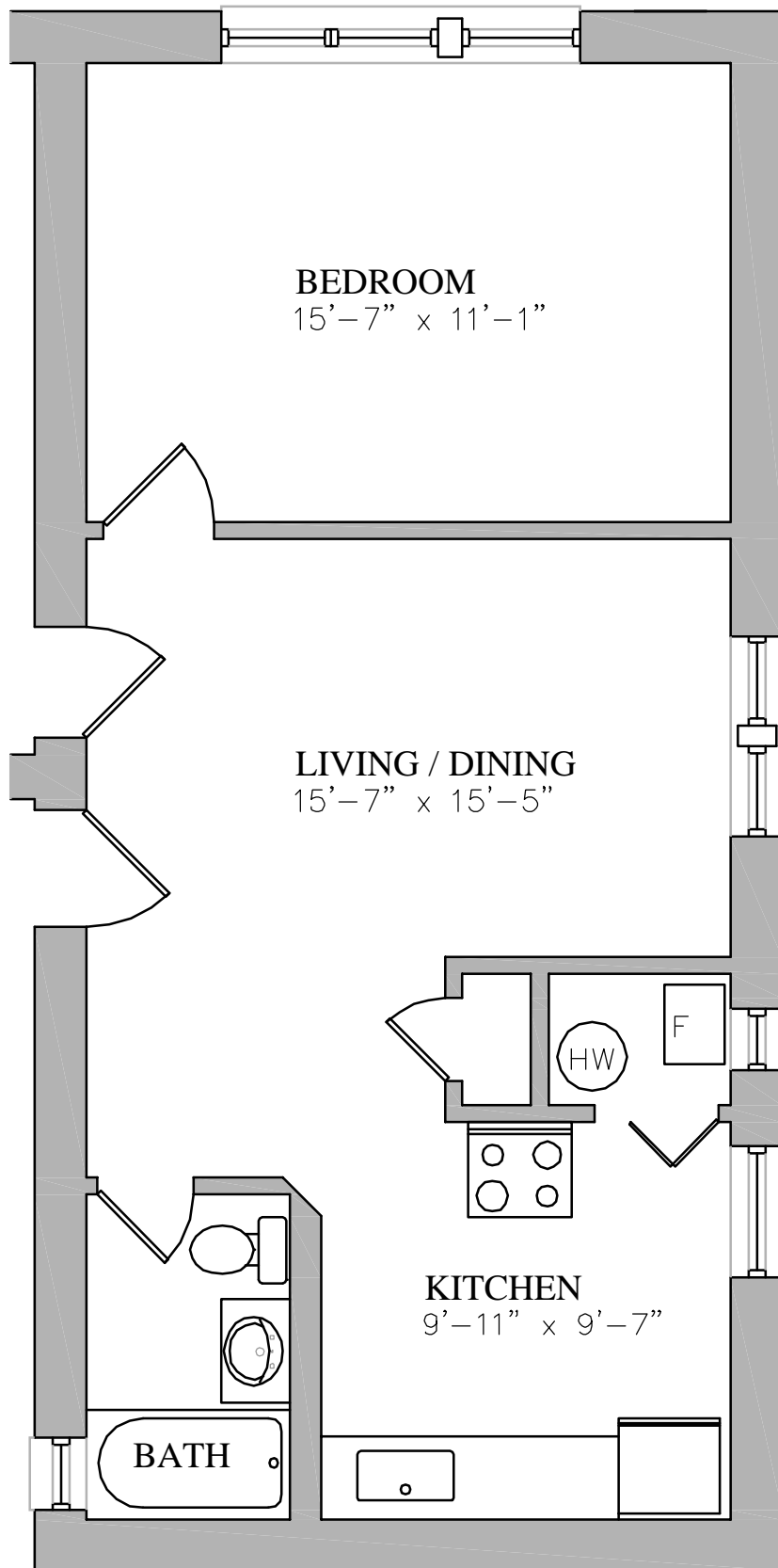
ONE-BEDROOM UNIT
